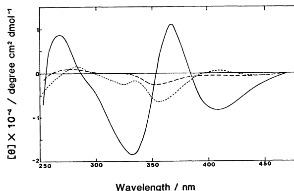
Fig. 7. CD spectra of bis(Dnp) derivatives of GS ( 31c ), 10a ( 31a ), and 10b ( 31b ) in MeOH. —: 31c , ---: 31a , .....: 31b .
